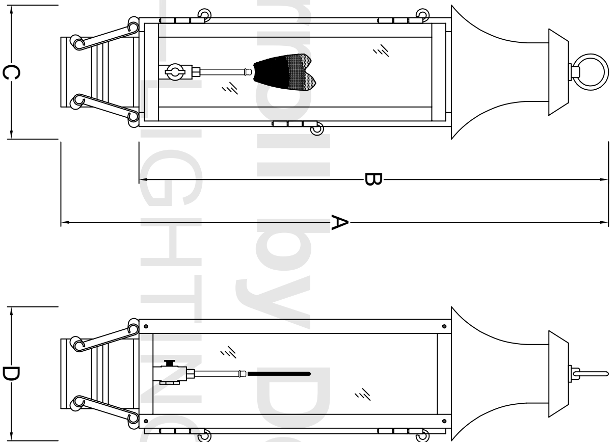
Front View
